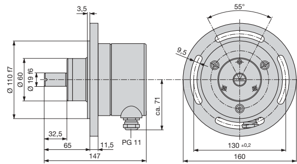
Fig. 8. KINAX WT 717 with flange.
