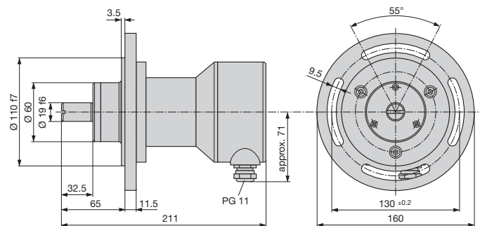
Fig. 10. KINAX WT 717 with additional gear and flange.
