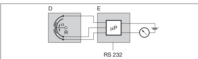
Fig. 2. Block diagram.
