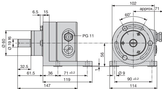
Fig. 7. KINAX WT 717 with foot.
