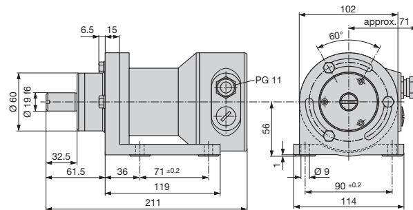
Fig. 9. KINAX WT 717 with additional gear and foot.
