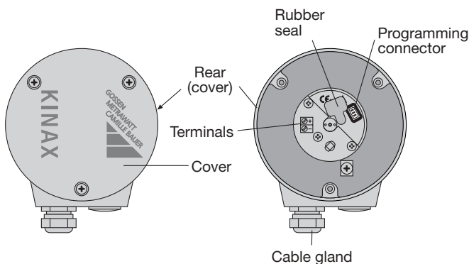
Fig. 5. KINAX WT 717 with screw terminals, programming connector and cable gland.
